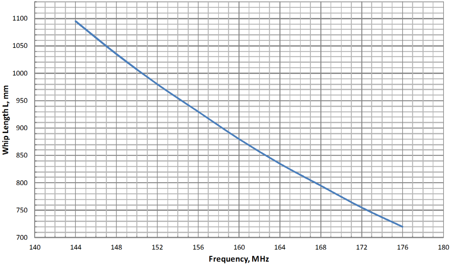
CELmar0T Tune Plot
